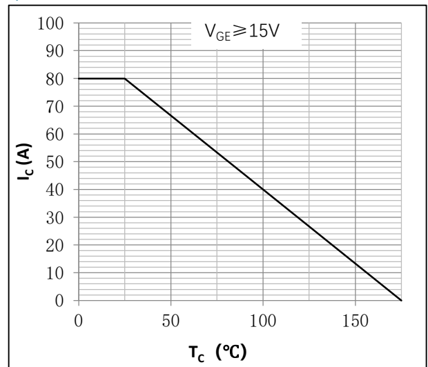
● Fig.6 Continuous collector current as a function of case temperature 1 ; Calculative values
